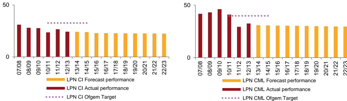
Figure 18 LPN's unplanned interruption and restoration performance
