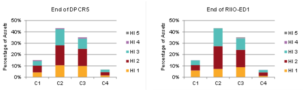
Figure 27 LPN Asset Criticality: % Assets by Criticality
