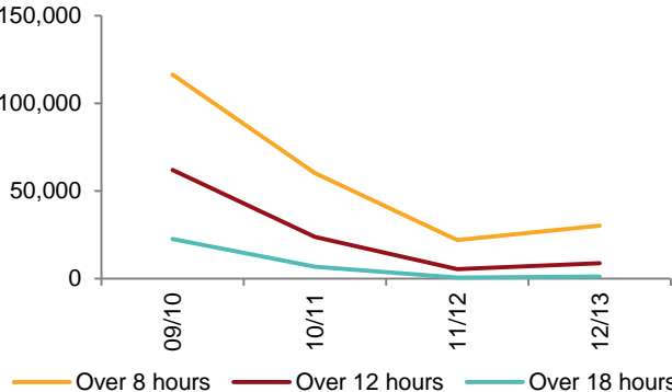
Figure 11 EPN 8, 12 and 18 hour interruptions
