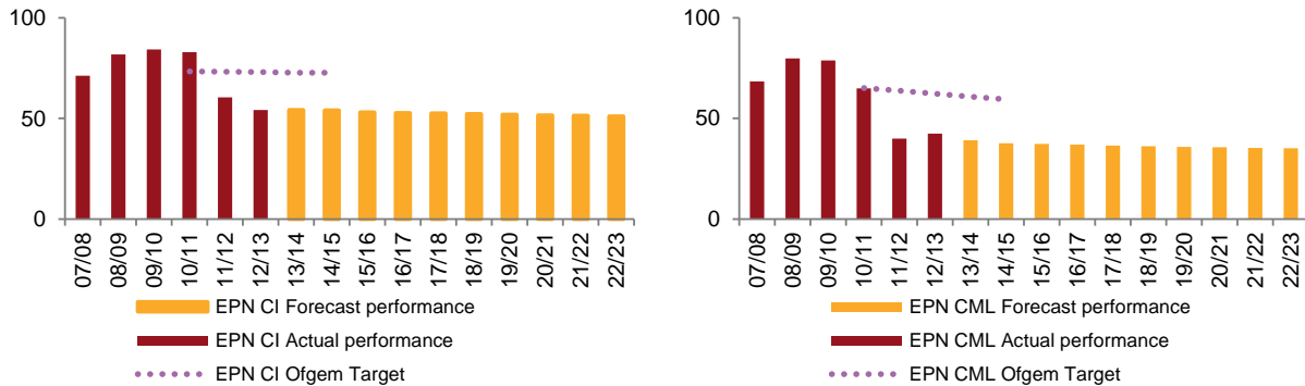
Figure 17 EPN's unplanned interruption and restoration performance
