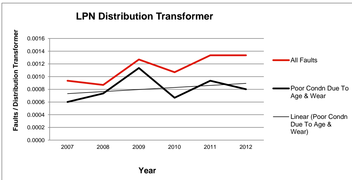
Figure 15 - Fault Rate Distribution Transformers in LPN (Source – 14th March 2013 UKPN Fault Cube)
