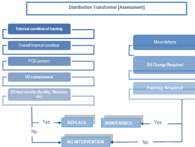
Figure 9 - Decision tree for interventions
