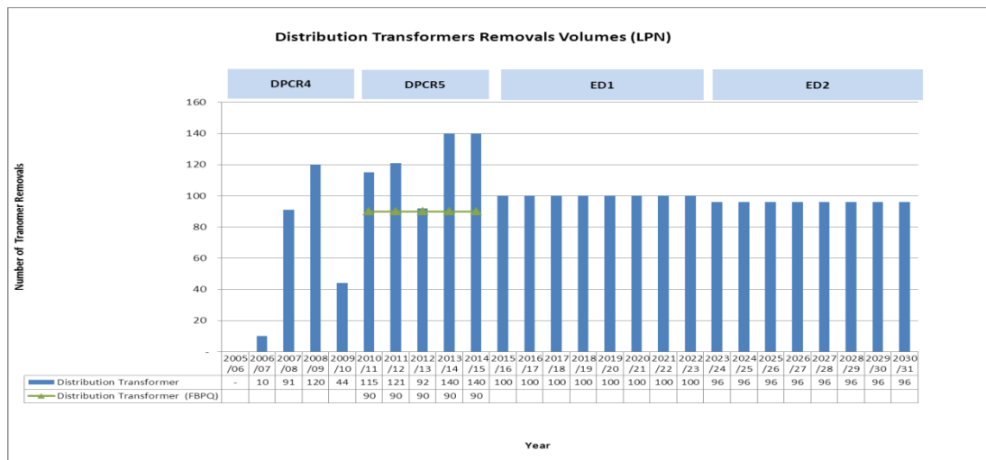
Figure 12: Distribution transformer removal volumes DPCR4 – ED2
