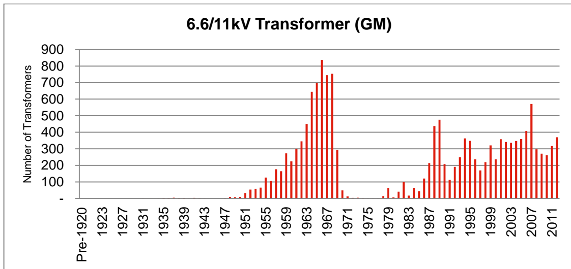
Figure 2: LPN Distribution Transformer Age Profile (Source – RIGS 2012 CV3 Table V5)
