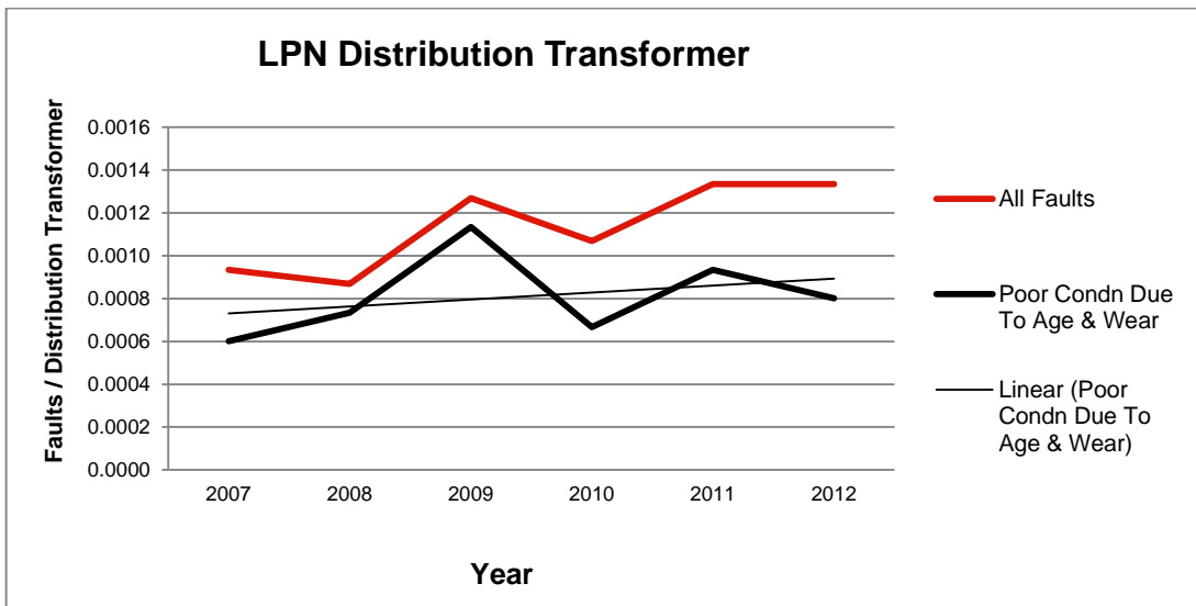
Figure 5 - Fault Rate Distribution Transformers in LPN (Source – 15 March 2013 UKPN Fault Cube)
